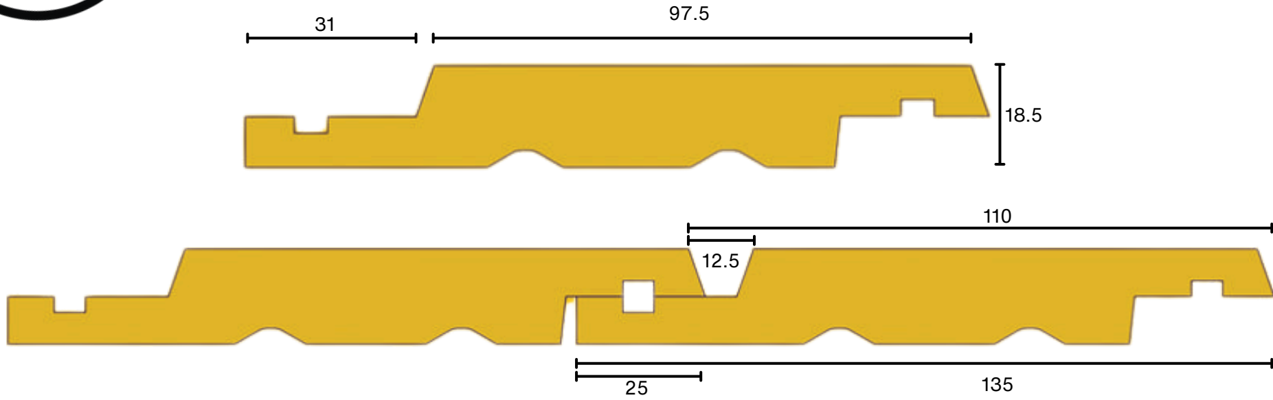
MD51 Vertical Shiplap 135/18.5mm 110mm Cover
